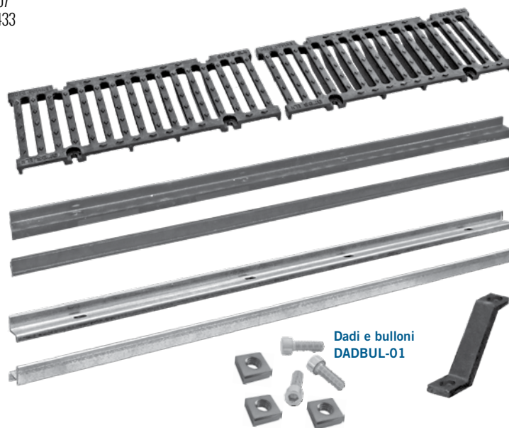
Griglia in ghisa GC25X50
